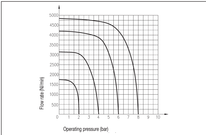
PILOT ACTUATED VALVES SIZE 1
